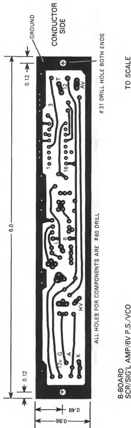
Figure 47. B circuit board, probe electronics.
